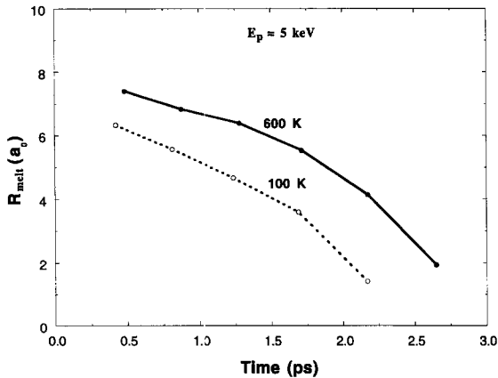
Fig. 7. Data for R_{melt} defined in the text as a function of time for T_{irr} = 100 K and 600 K.
