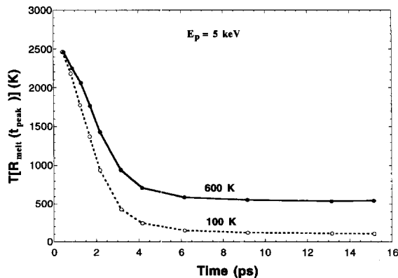
Fig. 8. The variation with time of the temperature in the sphere of radius R_{melt} at t_{peak} for T_{irr} = 100 K and 600 K.
