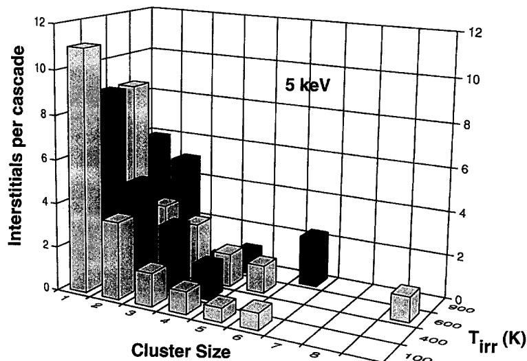
Fig. 10. Data for the number of interstitials per cascade in clusters of given size for each initial crystal temperature for PKA energy of 5 keV.
